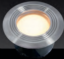
Onyx 60 R1 151D SMD LED 1W - A+ 2.700 K - 23 lm Edelstahl 47 x 75 mm (HxW) 1 m Kabel
